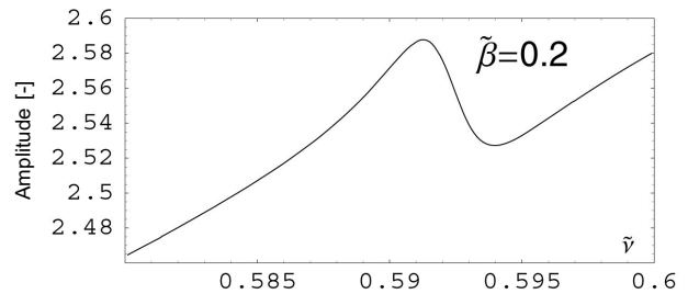
Fig. 9. Magnified region of frequency characteristic in the neighborhood of first resonance
