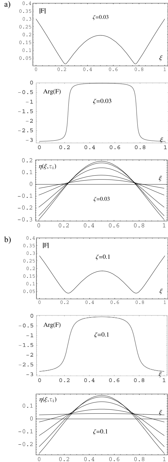
Fig. 4. Modulus and phase shift of the system response versus excitation and the effect of "moving antinodes" for damping \zeta = 0.03 and \zeta = 0.1 ((a) and (b) respectively)
