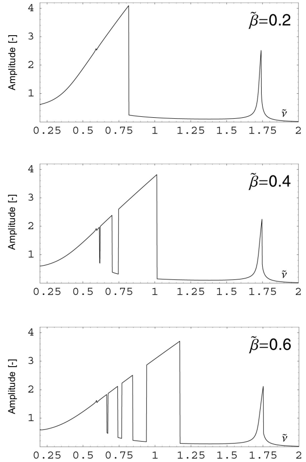
Fig. 8. Frequency characteristics for different values of nonlinearity
