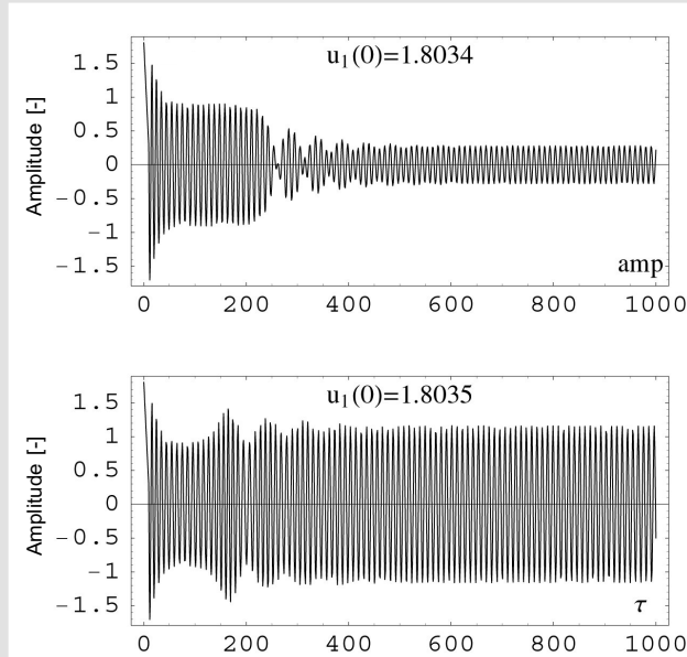
Fig. 7. Influence of the initial condition on the amplitude of steady-state
