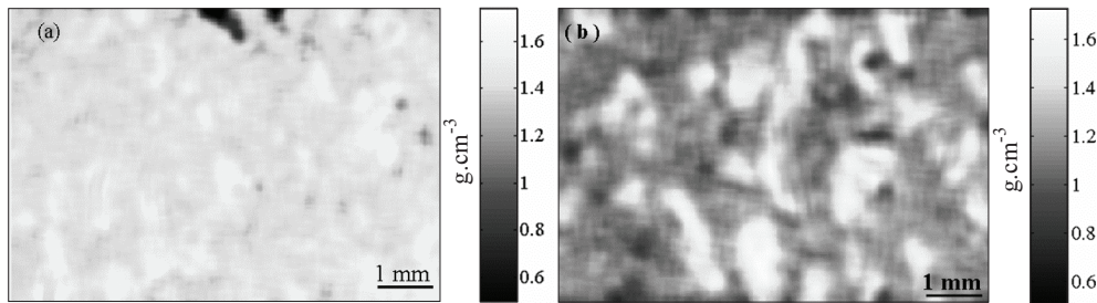
Fig. 3. Density maps of: a) virgin graphite; b) thermally oxidized graphite (weight loss of \sim 23\% ). Kernel box size: 286\text{ }\mu\text{m}
