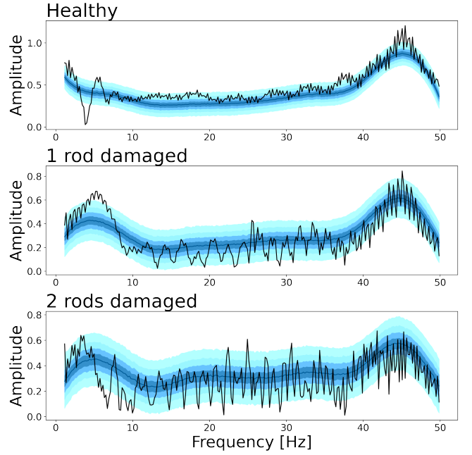
Fig. 4. To generate diverse data for training the classifier, we constructed models representing the magnitude response of each signal class using spline representation. We assumed a normal distribution for each spectrum. The figure showcases ribbon plots for different quantiles, with the median displayed in the center. Additionally, to provide a comparison, an example of the Fast Fourier Transform (FFT) from one of the signal classes is included.
