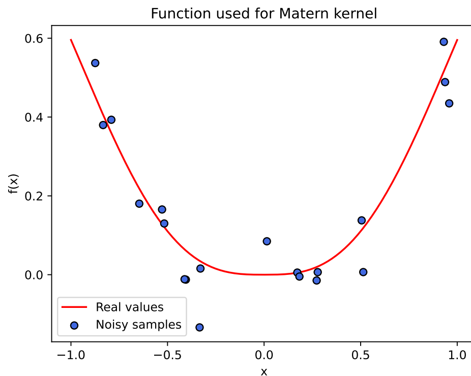
Figure 4. The plot shows an example of the twice differentiable function (red line) with sampled noisy values (blue) used for model fitting.
