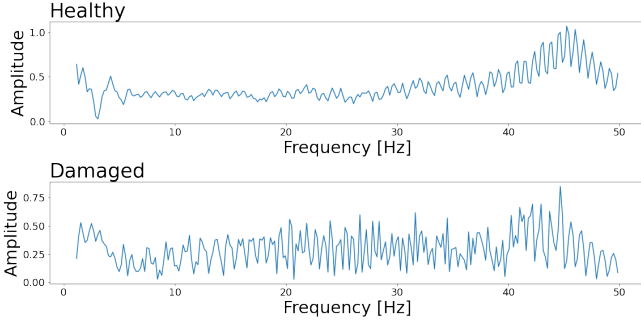
Fig. 3. Comparison of Fourier transforms of two example signals, after filtration and cutting off frequencies over 50 Hz.
