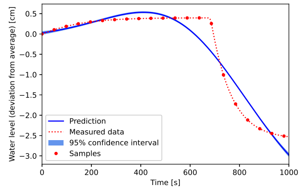
Fig. 5. Example of Gaussian Process fitted in faulty samples with usage of optimized hyperparameters for kernel. Red dots represent samples used in fitting process and red dashes the complete data set of measured data (the real trajectory of example). Blue line and field shows expected value (prediction) and confidence interval of predicted data. Prediction does not fit real trajectory with high accuracy and sometimes mismatches even out of shown confidence interval. This is caused due to set of hyperparameters, which were especially optimized to predict healthy trajectories, but it does not detract from the usefulness of GP for generating desired samples.
