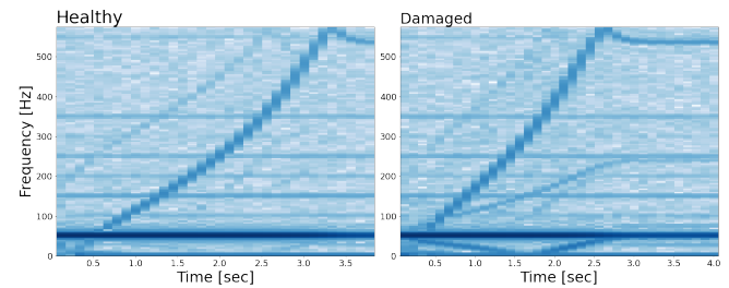
Fig. 2. Comparison of spectrograms of two example unfiltered signals. Components caused by rotational speed and supply frequency are identical in both healthy and damaged signals, however, we can see differences in the lower band.
