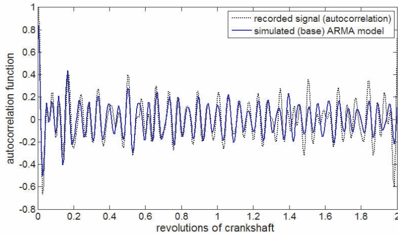
Fig. 8. Identification of the ARMA reference model of the gearbox vibration signal
