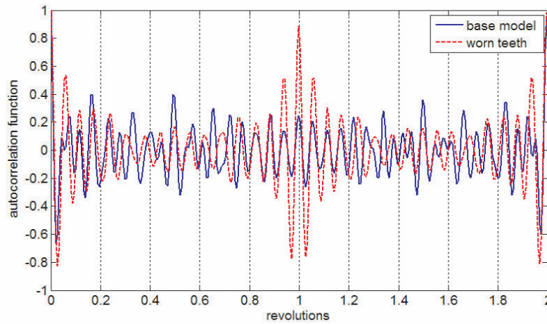
Fig. 9. Comparison of the reference model and the signal for the defective gearbox
