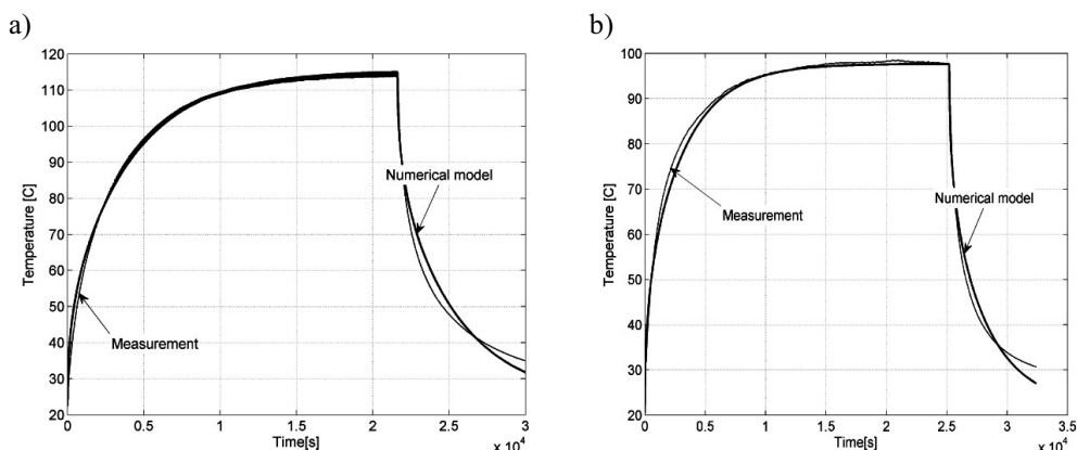
Fig. 3. Comparison of measured temperature step-input response and derived from the numerical model (a) for 6 rpm; b) for 120 rpm of rotation speed)
