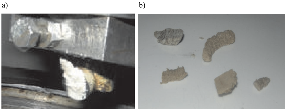
Fig. 6. Cuttings stuck to the cutter (Carthage Marble) (a), Ribbon shaped (Saw Tooth Shaped) cuttings (b)
