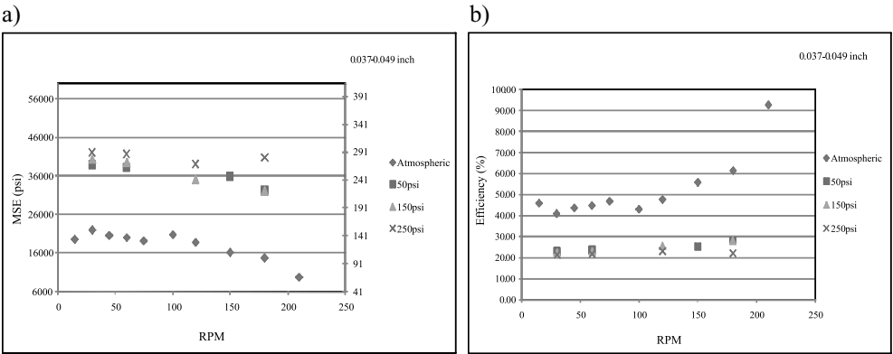
Fig. 10. MSE values (a) and efficiency of cutting (b) for tests performed on Carthage Marble as a function of RPM under varying borehole pressure
