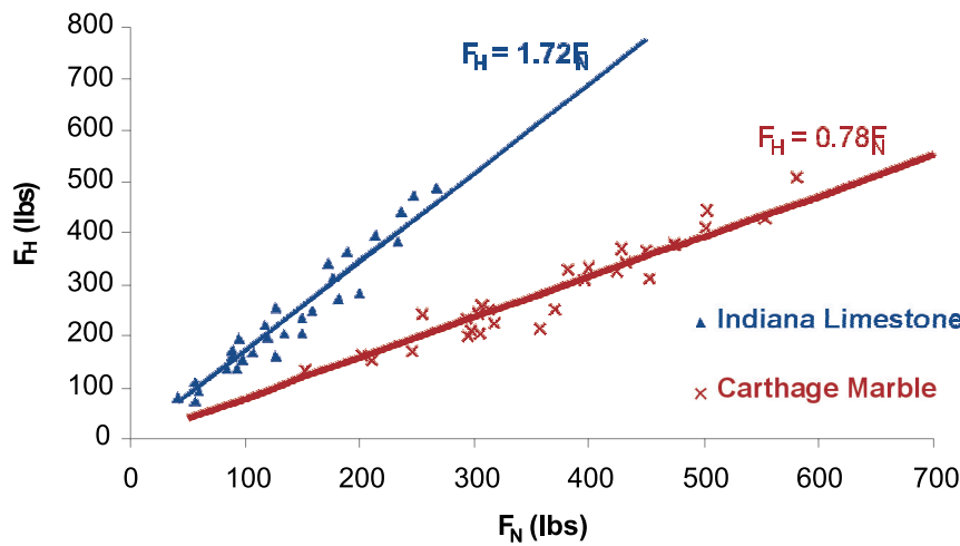
Fig. 14. Horizontal/ Cutting force ( F_H ) vs. Vertical/ Normal force ( F_N ) for tests on Indiana Limestone and Carthage Marble rock samples
