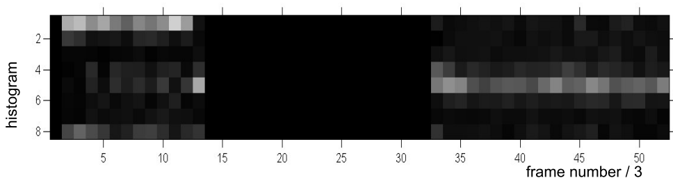
Fig. 3. Representation of the movie part by means of histograms of optical flow directions calculated for the every third frame. Motion to the right side of the scene corresponds to histogram bin equal to 1, motion to the left – bin equal to 5. Frames 1–13 – a person is running to the right, 14–32 – the scene is empty, 33–52 – a person is walking to the left
