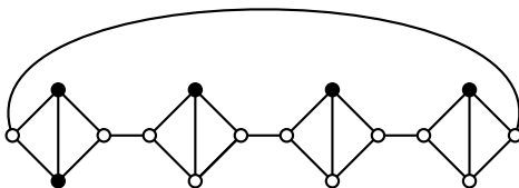
Fig. 6. The diamond-necklace N_4 and a 2-percolating set of size 5
