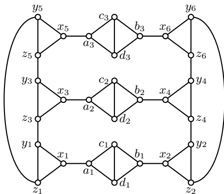
Fig. 3. The triangle-diamond-necklace H_6
