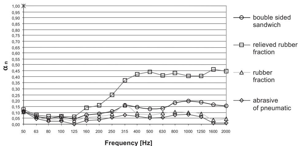
Fig. 5. Noise absorption coefficient of investigated acoustic patterns
