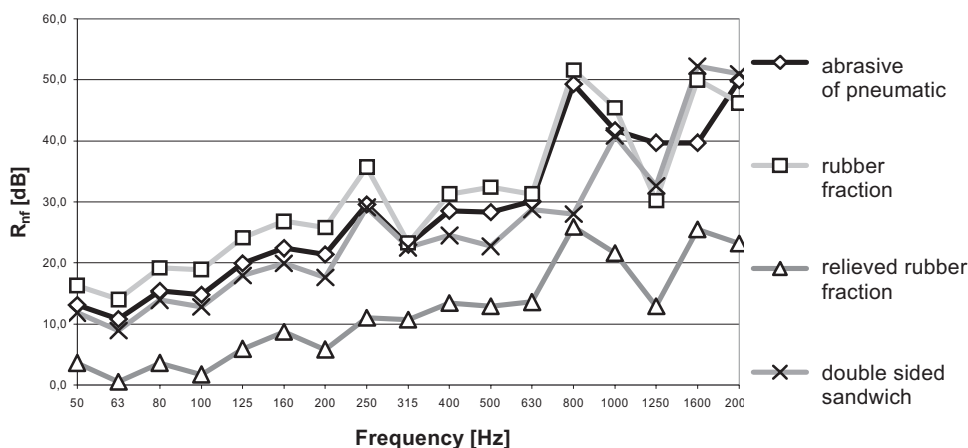
Fig. 7. Noise isolation coefficient of investigated acoustic patterns
