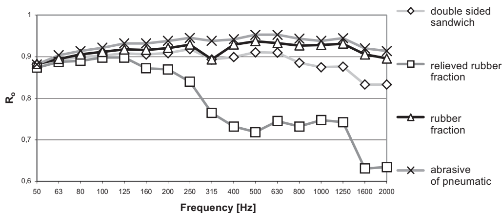
Fig. 6. Noise reflection coefficient of investigated acoustic patterns
