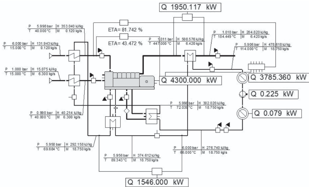
Fig. 2. Model engine CG 260 16V [3]
