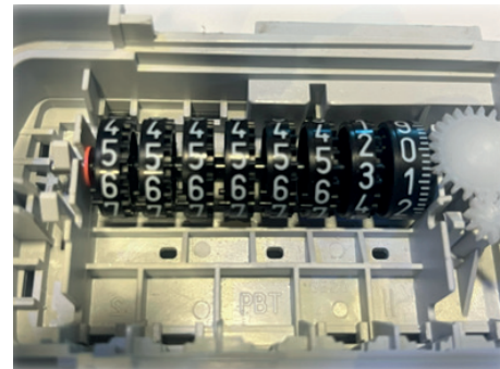
Fig. 13. The position of the teeth initiating the shifting of the “older” drum for drums indicating the number 0
