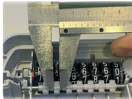
Fig. 12. The width of the wider tooth of the decade flip-flop (4 mm)
