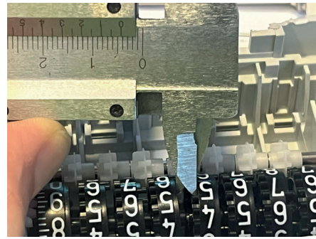
Fig. 11. The distance from the drum to the tooth cavity (4.30 mm)
