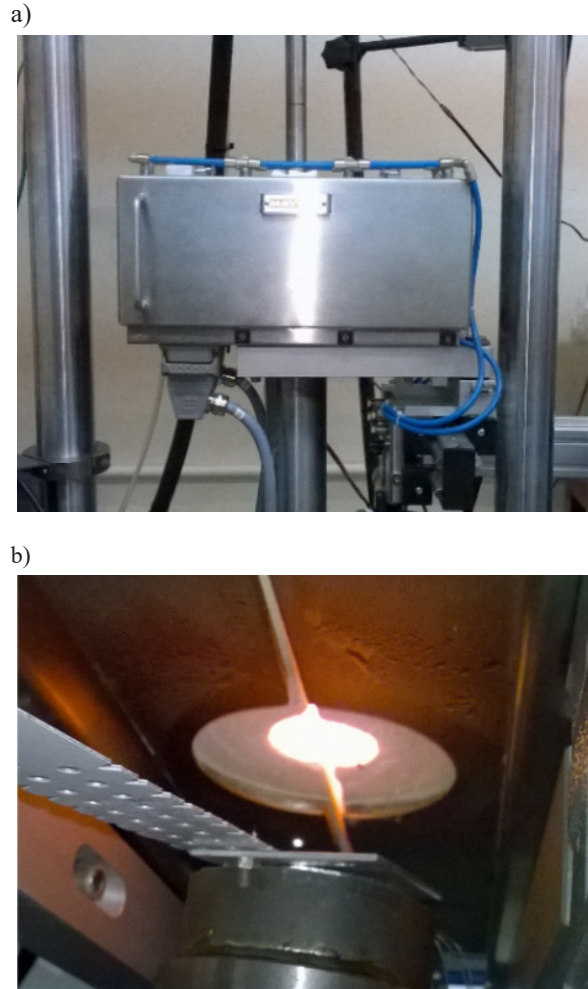
Fig. 4. View of the measurement station: a) heating furnace; b) cold sample protected with a thermal shield
