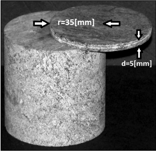
Fig. 3. The photo of the migamtites sample preperd to the thermal conductivity coefficient
