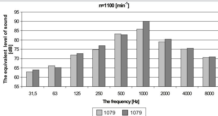
Fig. 7. The dependence of equivalent levels of sound on frequency for disintegration of andesite
