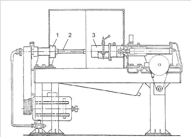
Fig. 1. The scheme experimental drilling stand
