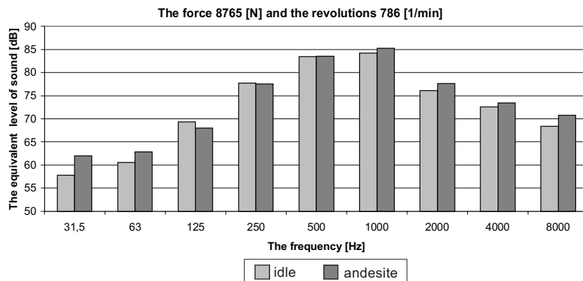
Fig. 8. The comparing of equivalent levels of sound at various frequencies in idle mode and during andesite disintegration
