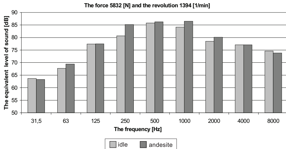
Fig. 10. The comparing of equivalent levels of sound at various frequencies in idle mode and during andesite disintegration
