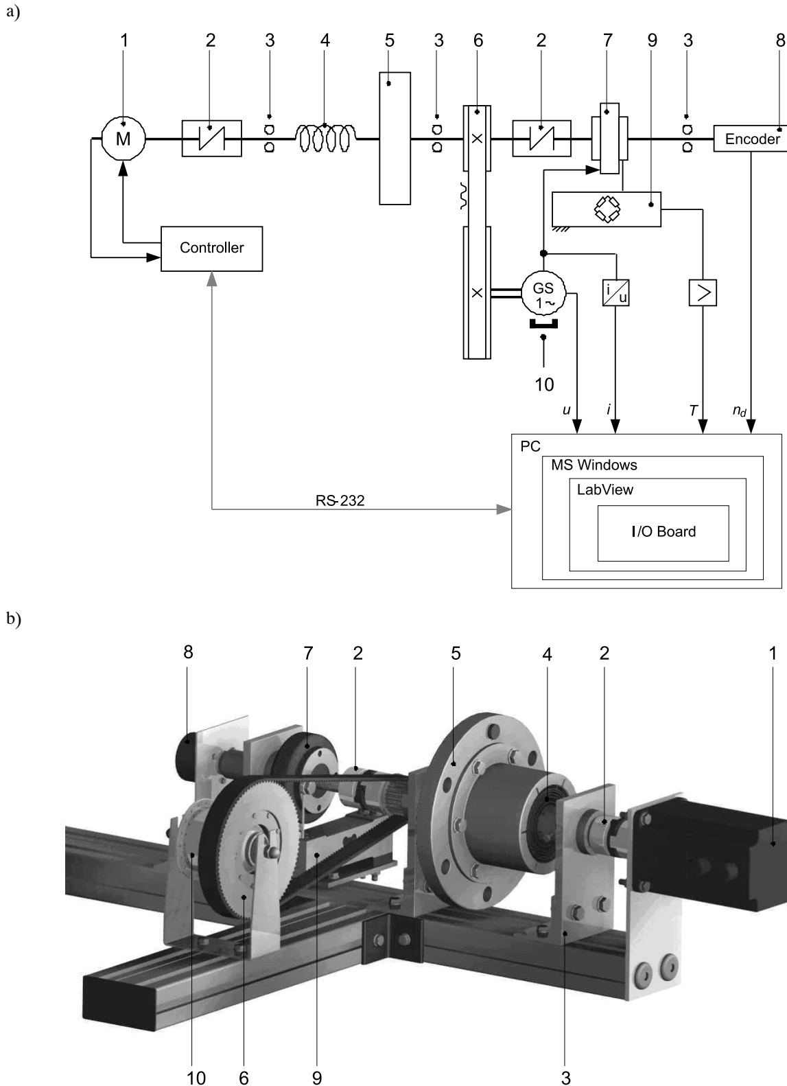
Fig. 2. Test bed: 1 – servomotor, 2 – clutch, 3 – bearing, 4 – spring, 5 – rotary disk, 6 – belt transmission, 7 – MR rotary damper, 8 – encoder, 9 – beam load cell, 10 – electromagnetic generator. Schematic diagram (a), general view (b)
