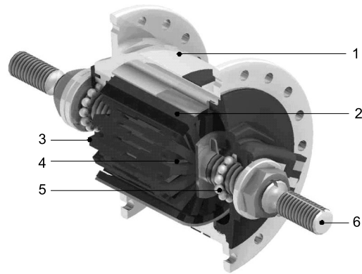
Fig. 5. Structure of the DH-3N30 generator: 1 – rotor, 2 – magnet, 3 – frame, 4 – coil, 5 – bearing, 6 – shaft
