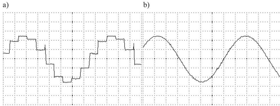
Fig. 7. The generated sin wave – oscilloscope screen: a) Voltage 2 V/div vs. time 50 μs/div; b) Voltage 2 V/div vs. time 0.5 ms/div
