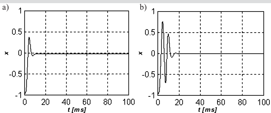
Fig. 4. Simulation results: a) startup without disturbance observer; b) startup with disturbance observer
