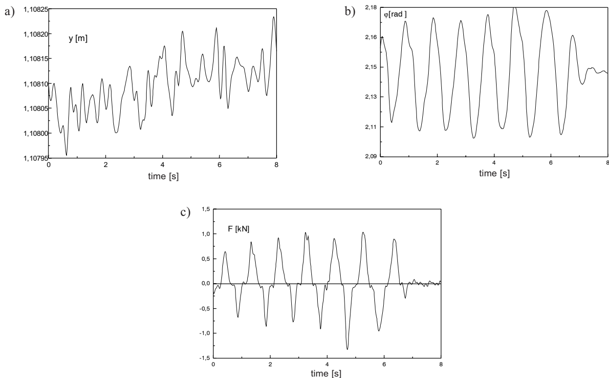
Fig. 8. Signals registered in the excavator elements: a) displacement of the servo-motor; b) angular rotation of the bucket; c) force acting on the servo-motor piston rod
