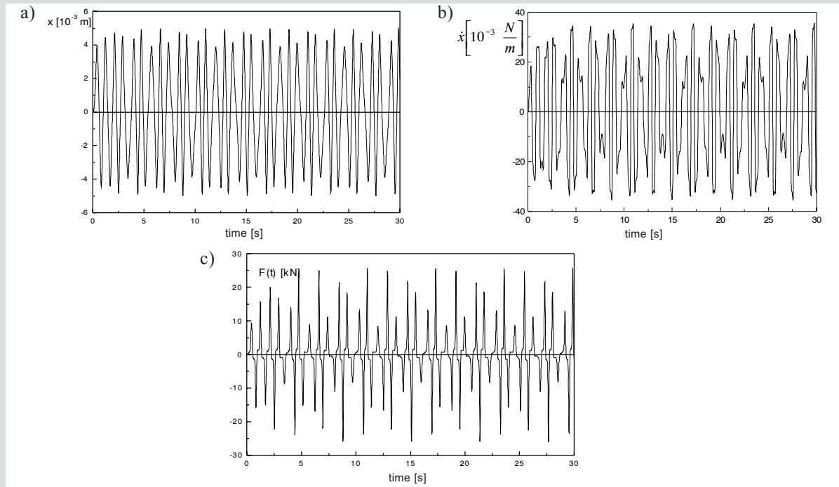
Fig. 5. The system response: a) displacement; b) velocity; c) force
