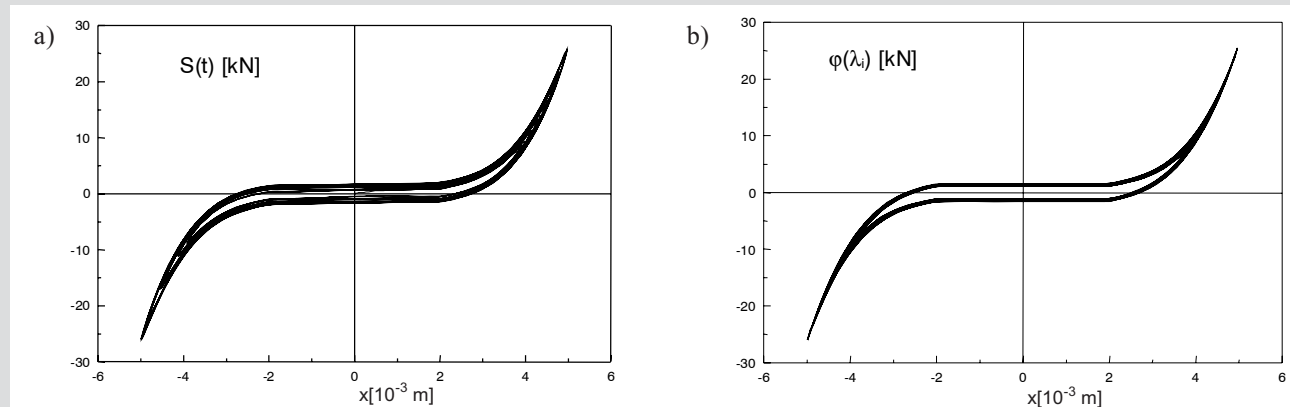
Fig. 6. Interaction force acting between: a) the system and the mass; b) the modelling function
