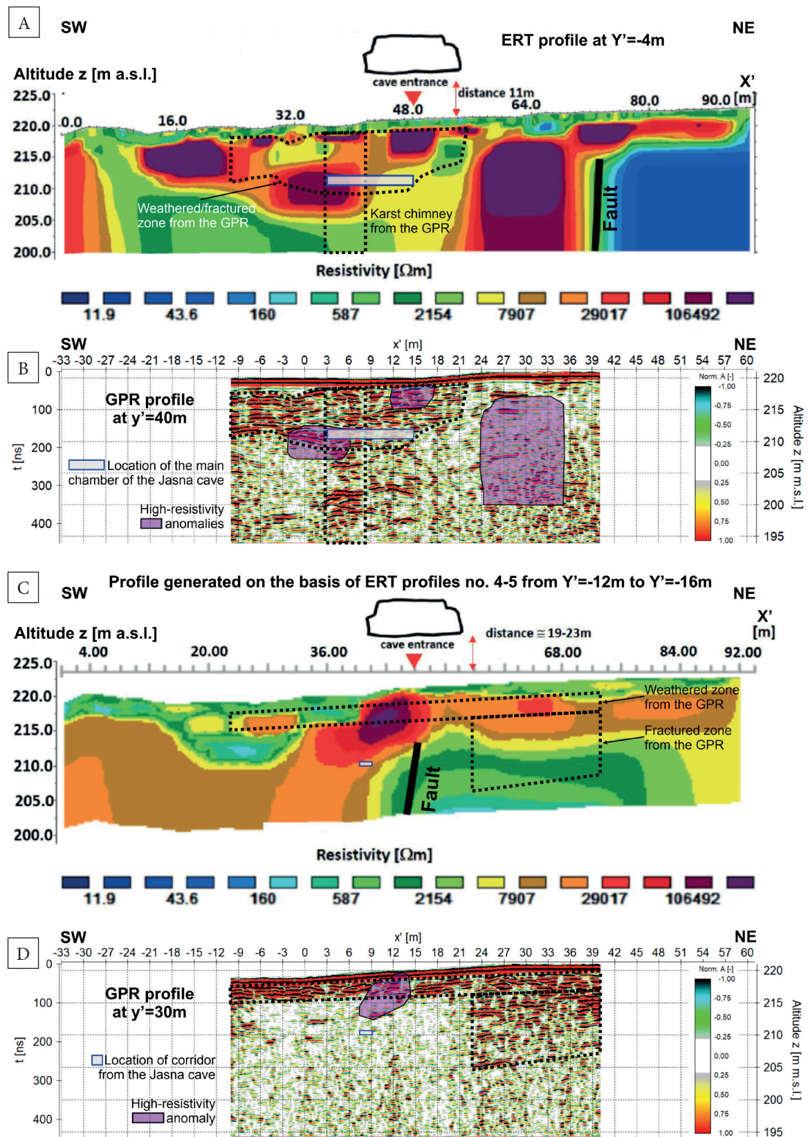
Fig. 16. Cross-section along profile ERT-2, obtained from the 2D inversion (Pasierb 2022 – modified) (A); y' cuts of 3D block (Fig. 12 – GPR results) at y' = 40\text{ m} (B); cross-section along profiles ERT-4 and ERT-5 obtained from the 3D inversion (Pasierb 2022 – modified) (C); y' cuts of 3D block (Fig. 12 – GPR results) at y' = 30\text{ m} (D)
