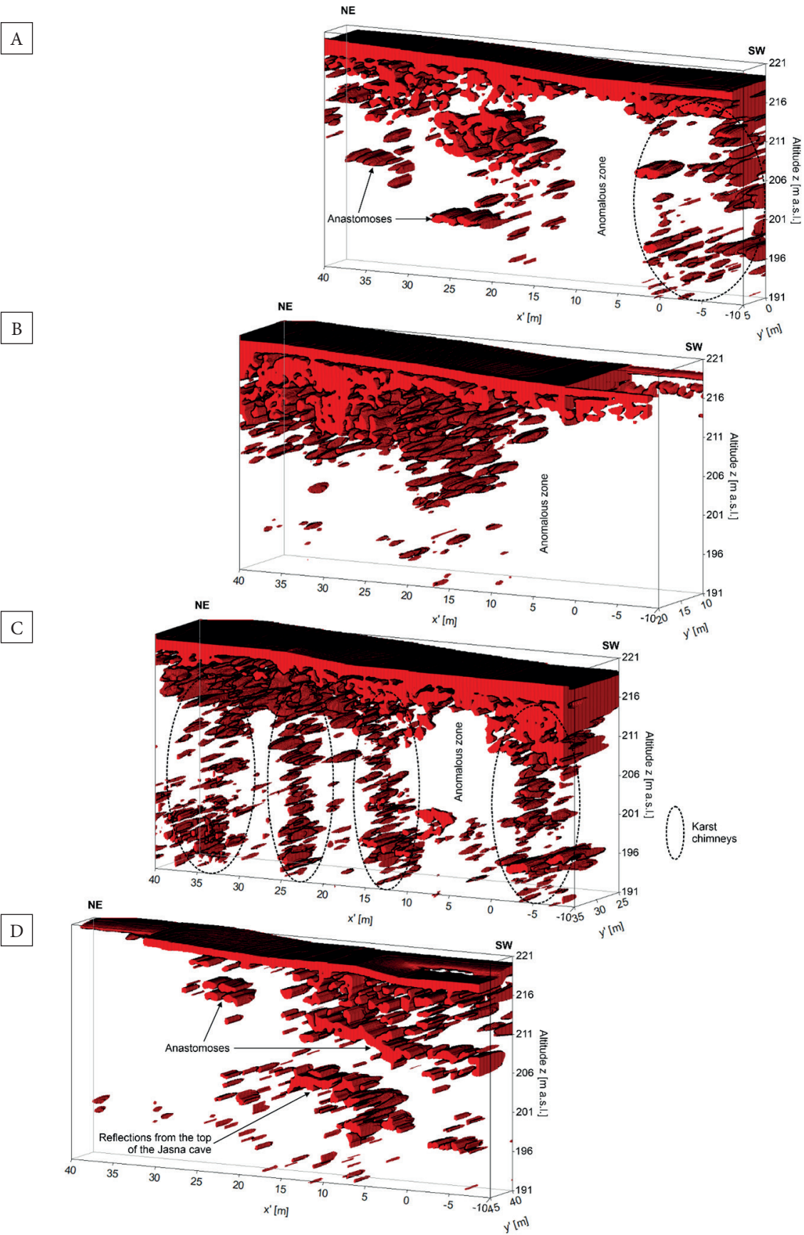
Fig. 12. 3D volumetric visualisation of the main GPR anomalies
