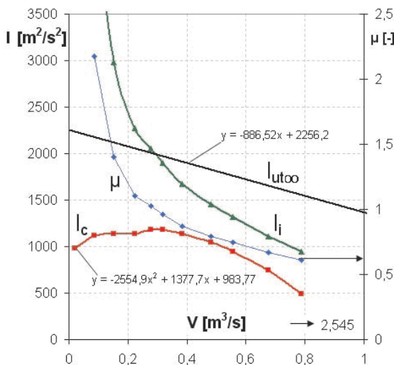
Fig. 4. Experimental characteristics l_c situated on the background of rotor work l_{ut\infty} , l_i , and \mu
