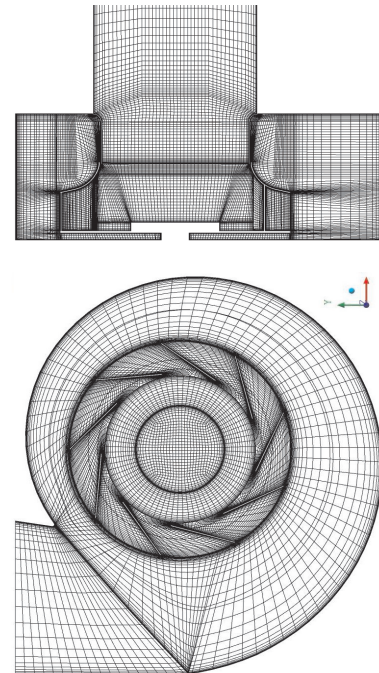
Fig. 7. Computational mesh
