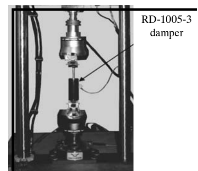
Fig. 7. RD-1005-3 damper in the Instron machine
