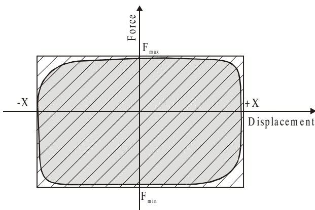
Fig. 5. Representation of energy dissipation by a MR damper over one cycle
