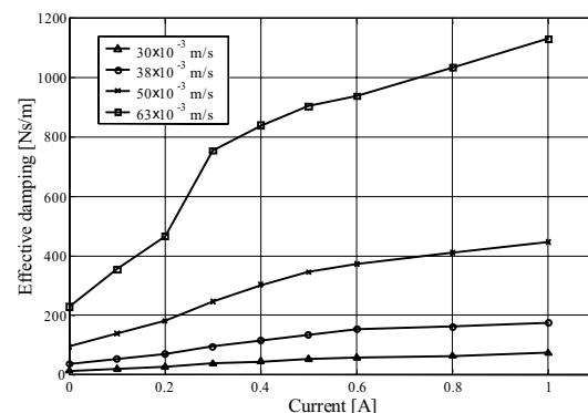
Fig. 11. Effective damping vs. current
