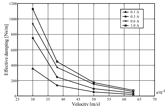
Fig. 13. Effective damping vs. velocity
