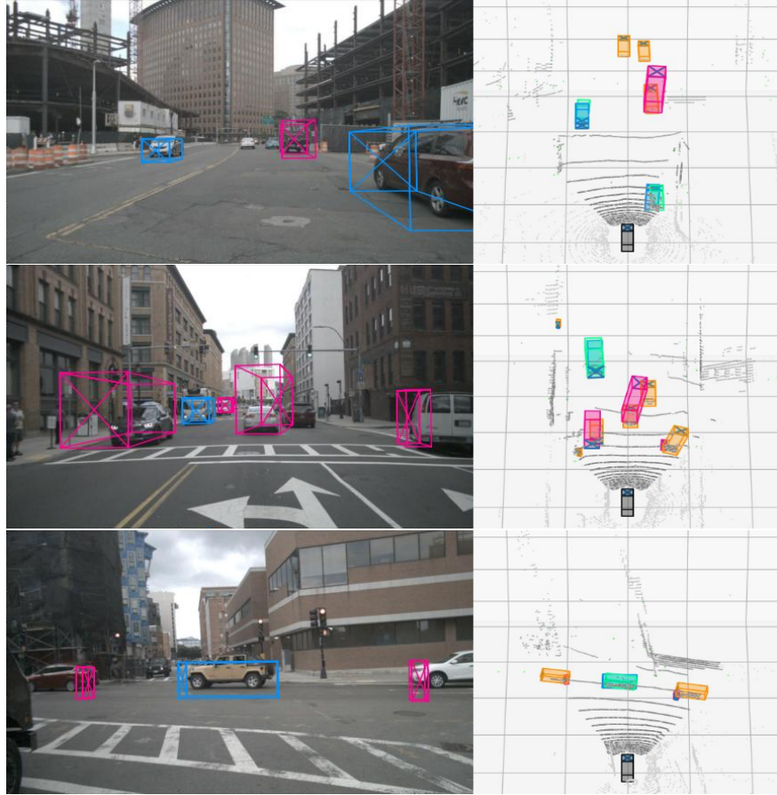
Figure 7.5: The results of Radar-only 3D OD model on NuScenes test set. The visualization overlay follows the same scheme, with labels, positive detections, false detections, and missed ones marked in green, blue, magenta and yellow respectively. Compared to previous experiments, Radar-only model provides significantly lower visual 3D OD results.
