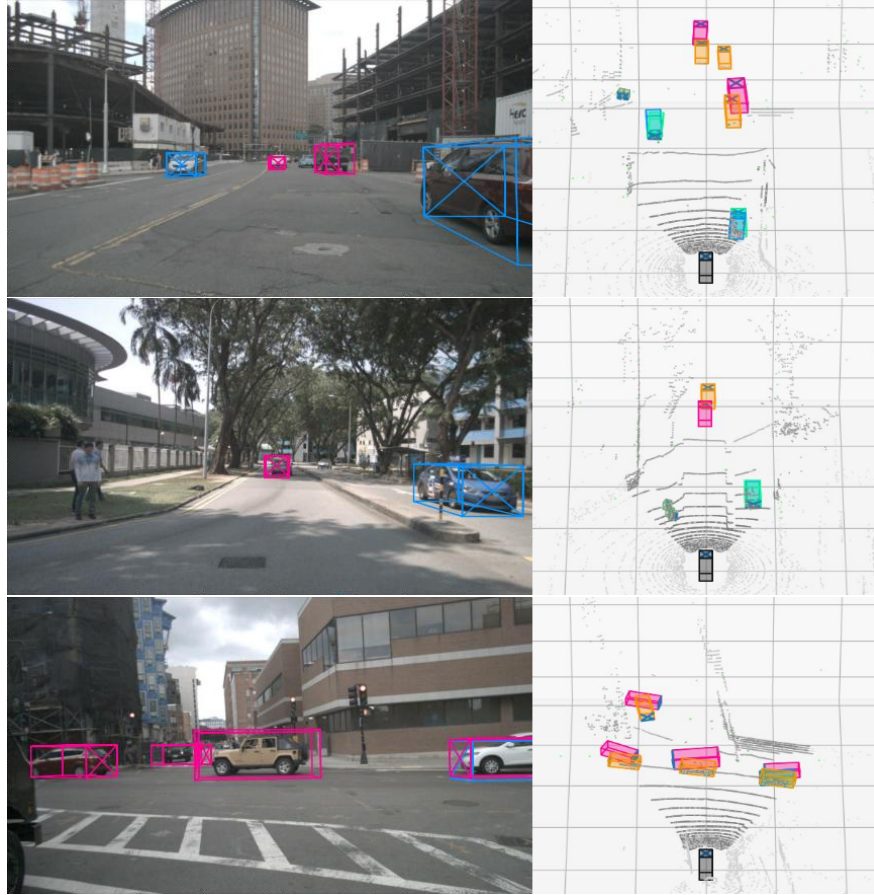
Figure 7.7: The results of monocular camera-only 3D OD model on NuScenes test set. The visualization overlay follows a previously introduced colour coding scheme: labels, positive detections, false detections, and missed ones are marked in green, blue, magenta and yellow respectively. The pointcloud data is added for enhanced BEV visualization, however, it was not used for obtaining the 3D predictions, which are based only on camera image.
