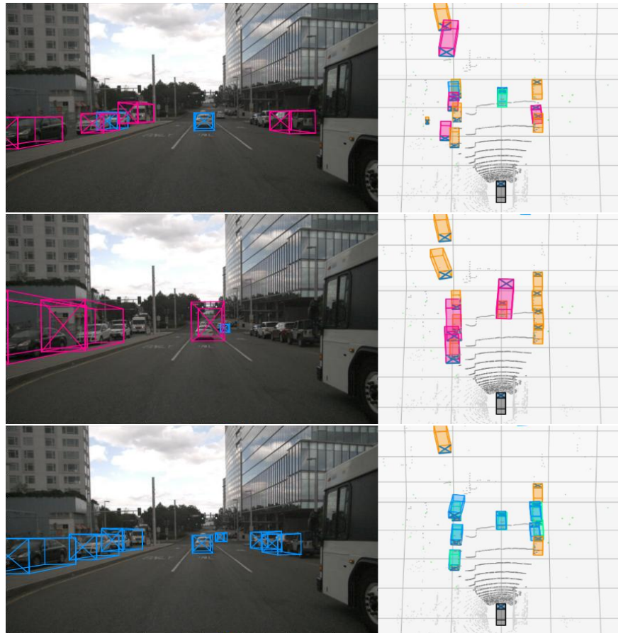
Figure 8.6: The comparison of another scene from the NuScenes test dataset, with predictions from the camera-only, radar-only, and CDSM fusion models respectively from top to bottom. The visualization overlay follows the described colour scheme: labels are shown in green, positive detections in blue, false detections in magenta, and missed detections in yellow. The image demonstrates the detection accuracy gain of the fusion approach with respect to both single-sensor models.
