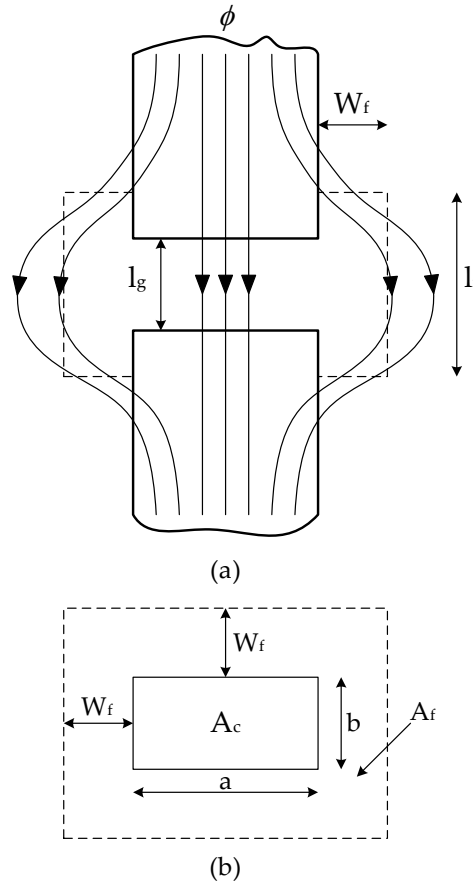
Figure 25: Kazimierczuk's Fringing Flux Calculation Method; (a) Flux Distribution Around the Air Gap; (b) Cross-Sectional Area of the Core A_c and the Fringing Flux A_f .
