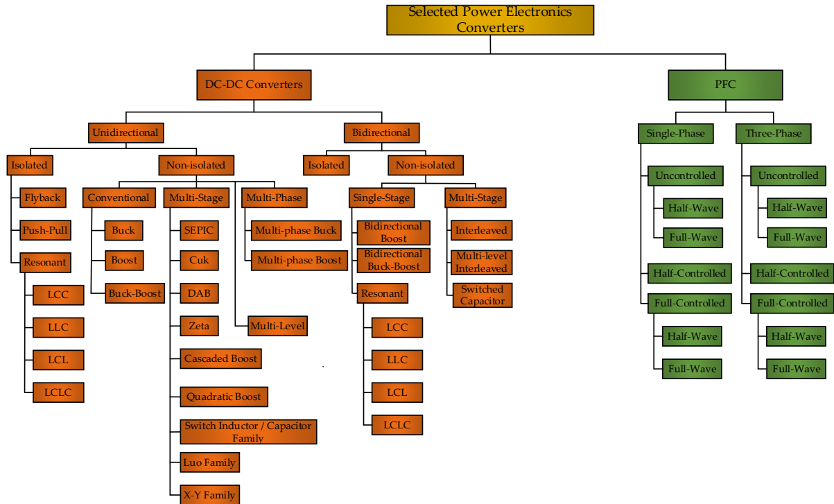
Figure 4: Classification of Selected Power Electronics Converters.
