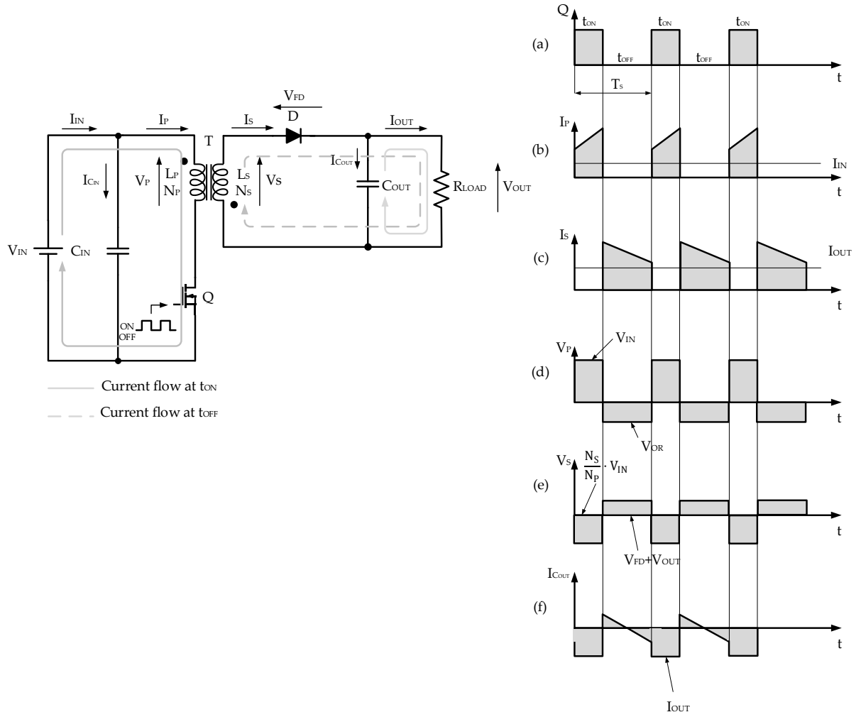
Figure 10: Flyback Converter Operation in Continuous Conduction Mode; (a) t_{ON} and t_{OFF} State of the Switch Q ; (b) Inductor Primary Current I_P ; (c) Inductor Secondary Current I_S ; (d) Inductor Primary Voltage V_P ; (e) Inductor Secondary Voltage V_S ; (f) Output Capacitor C_{OUT} Current.
