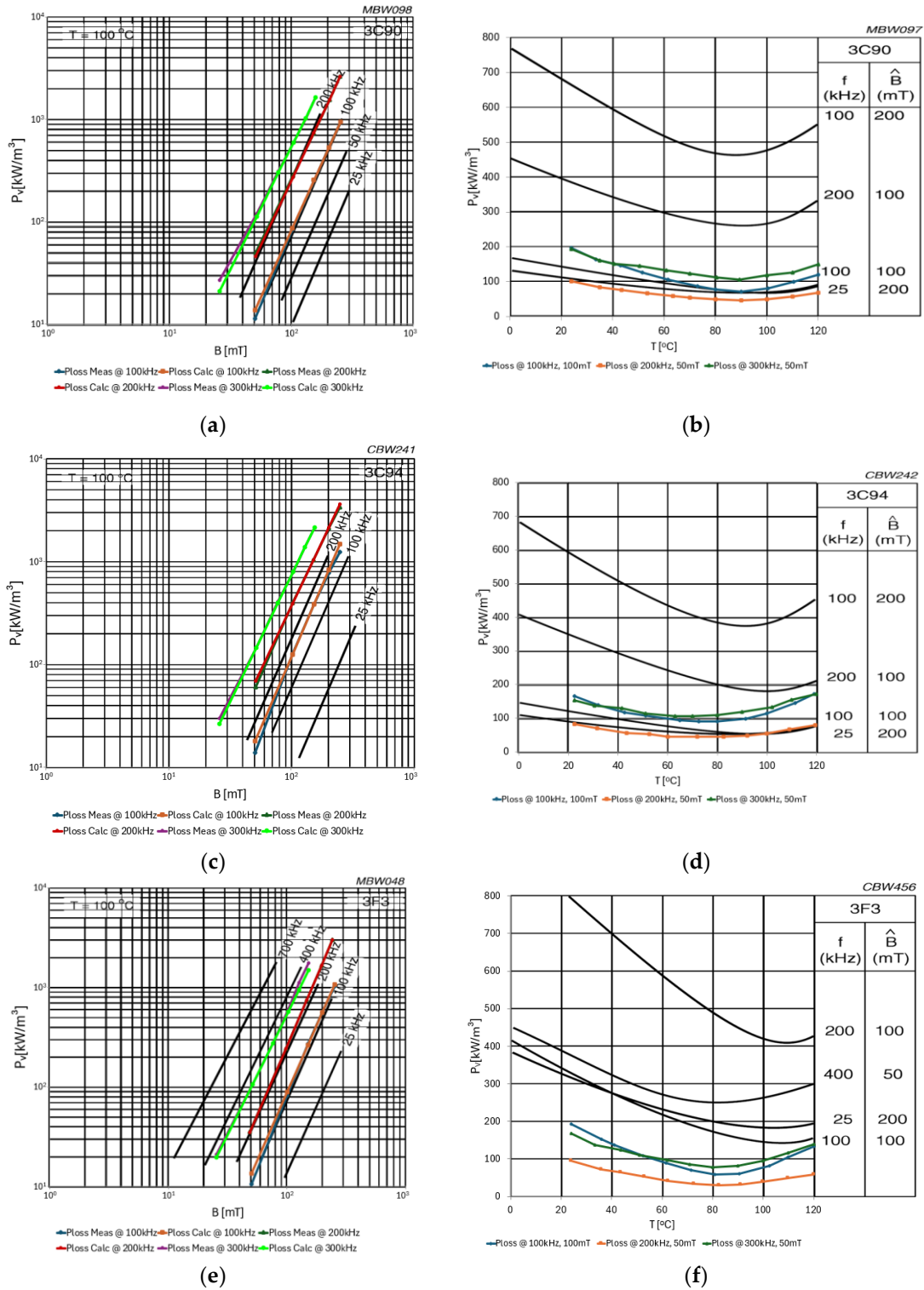
Figure 64: Fitting of Large-Signal Core Loss Characteristics under Sinusoidal Excitation Versus Magnetic Flux Density @ 100^\circ\text{C} and Versus Temperature: (a) Sample 7 P_v vs. B_m @ 100^\circ\text{C} , Blue – Measured Characteristics @ 100 kHz, Orange – Fitted Characteristics @ 100 kHz; Dark Green – Measured Characteristics @ 200 kHz, Red – Fitted Characteristics @ 200 kHz, Purple – Measured Characteristics @ 300 kHz, Light Green – Fitted Characteristics @ 300 kHz; (b) Sample 7 P_v vs. T , Blue - @ 100 kHz and 100 mT Signal Swing, Orange - @ 200 kHz and 50 mT Signal Swing, Green - @ 300 kHz and 50 mT Signal Swing; (c) Sample 8 P_v vs. B_m @ 100^\circ\text{C} , Blue – Measured Characteristics @ 100 kHz,
