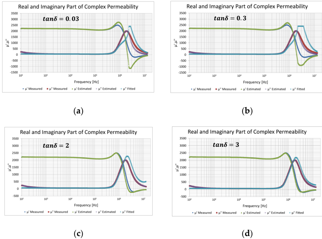
Figure 49: Sample 2 Fitting Convergence Depending on Loss Tangent Value, Dark Blue – Real Part of Measured Characteristic, Green – Real Part of Estimated Characteristic, Dark Red – Imaginary Part of Measured Characteristic, Purple – Imaginary Part of Estimated Characteristic, Light Blue – Imaginary Part of Fitted Characteristic; (a) Loss Tangent 0.03; (b) Loss Tangent 0.3; (c) Loss Tangent 2; (d) Loss Tangent 3.
