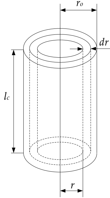
Figure 22: Cylindrical Magnetic Core Cross-Section.
