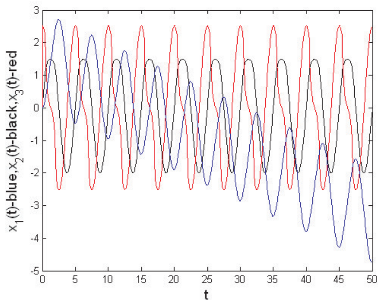
Fig. 7. Transient characteristics of the second order system (9)–(10) with asymmetry
