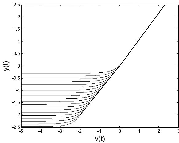
Fig. 3. Static characteristics of the non-symmetric saturation element
