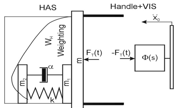
Fig. 4. The exemplary hybrid HAS model with handle and VIS
