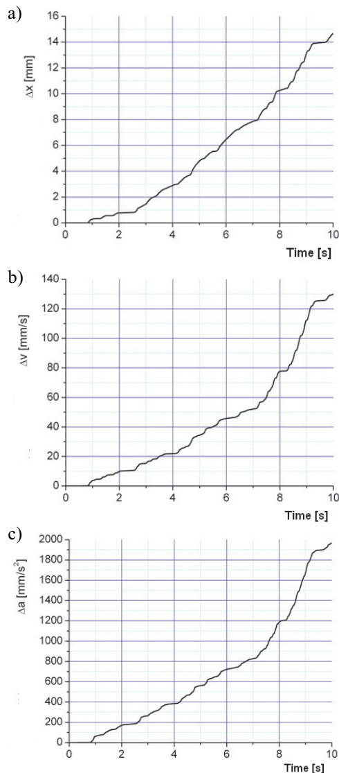
Fig. 9. Experimental values of absolute follow-up error signal of position \Delta x (a), velocity \Delta v (b) and acceleration \Delta a (c)
