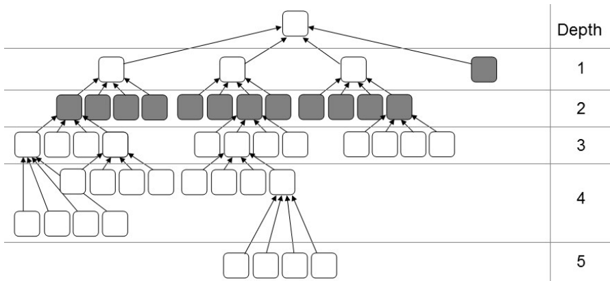
Fig. 4. Quad tree structure with example of nodes chosen while rendering terrain with LoD enabled
