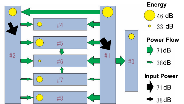
Fig. 6. Energy transfer path at the 500 Hz 1/3 octave band frequency during printing
