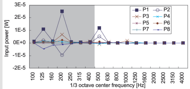
Fig. 5. Identified power input during printing
