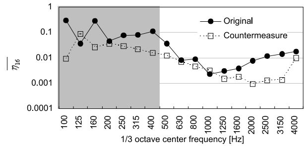
Fig. 9. Comparison between the original and the countermeasure values of the coupling loss factor from the 1st to the 6th subsystem
