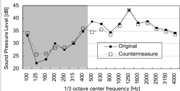
Fig. 10. Comparison of the sound pressure levels with and without the countermeasure
