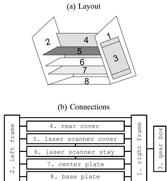
Fig. 3. Subdivision of the test printer
