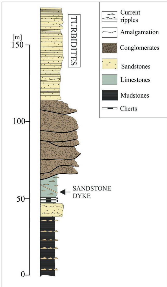
Fig. 19. Schematic section of the lithological succession at Skrzydlina quarry
