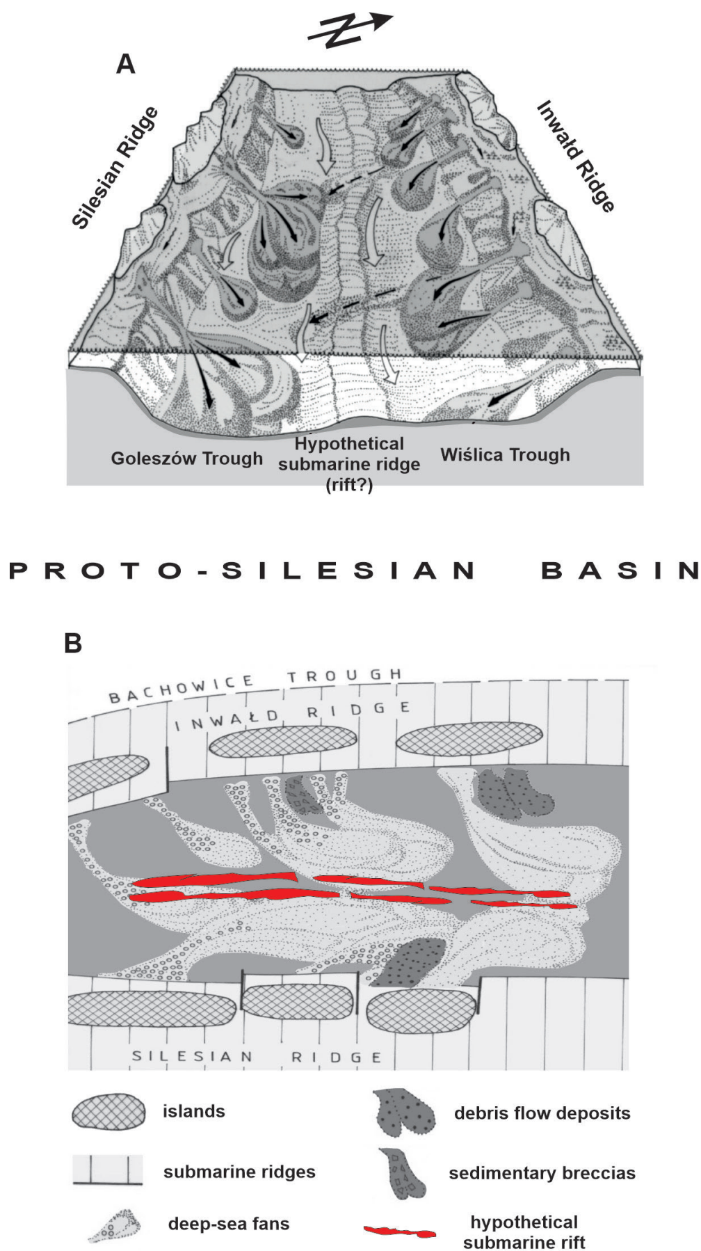
Fig. 54. Palaeogeographical blockdiagram of sedimentation of the oldest flysch deposits in the Proto-Silesian Basin (Jurassic/Cretaceous transition – Tithonian/Berriasian) (A) and its hypothetical palaeogeographical sketch (B) (after Słomka 1986a; slightly modified)
