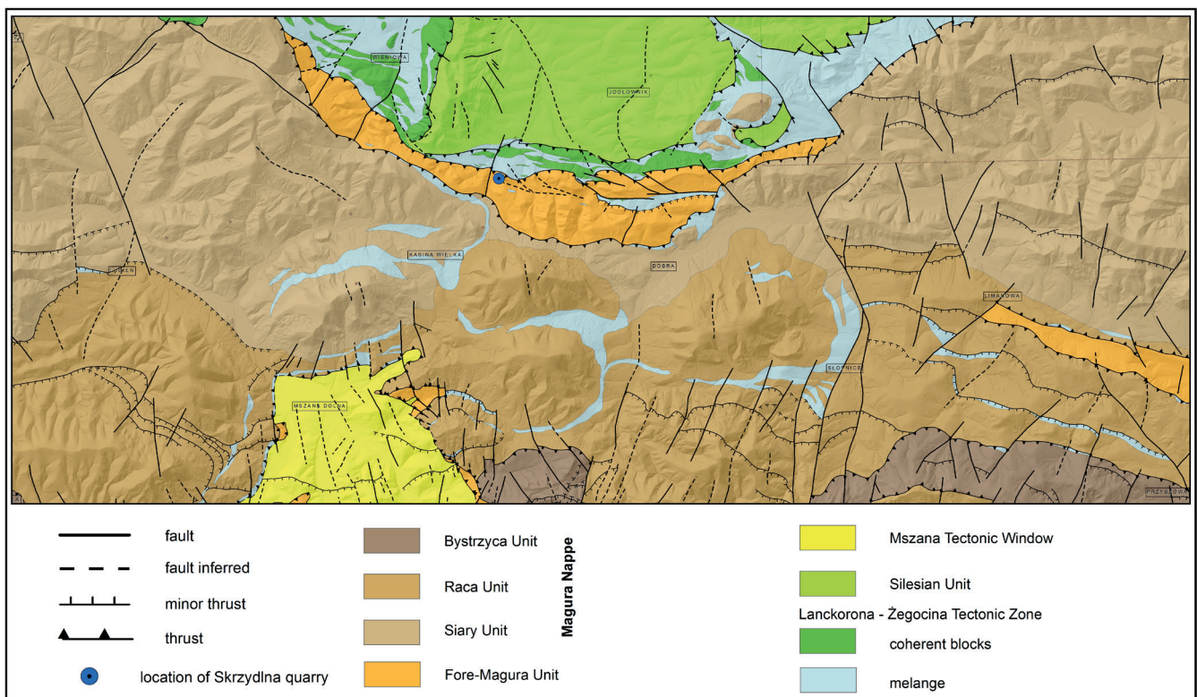
Fig. 15. Regional tectonic sketch with the location of the Skrzydlina quarry (based on Żytka et al. , 1989, modified)
