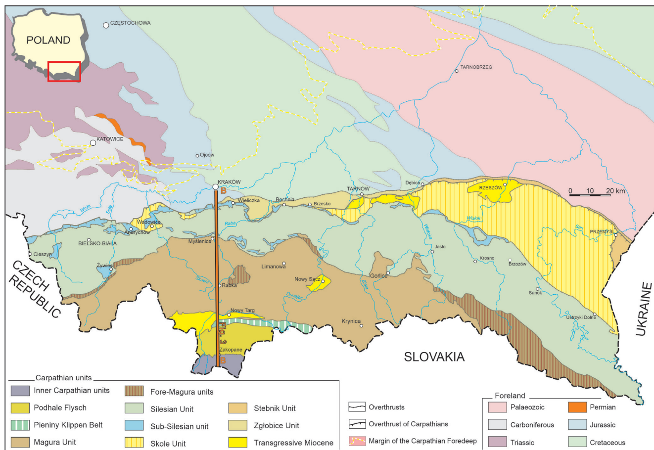
Fig. 4. Geological map of the Polish Carpathians and Foreland (after Żytko et al. , 1989; simplified)
