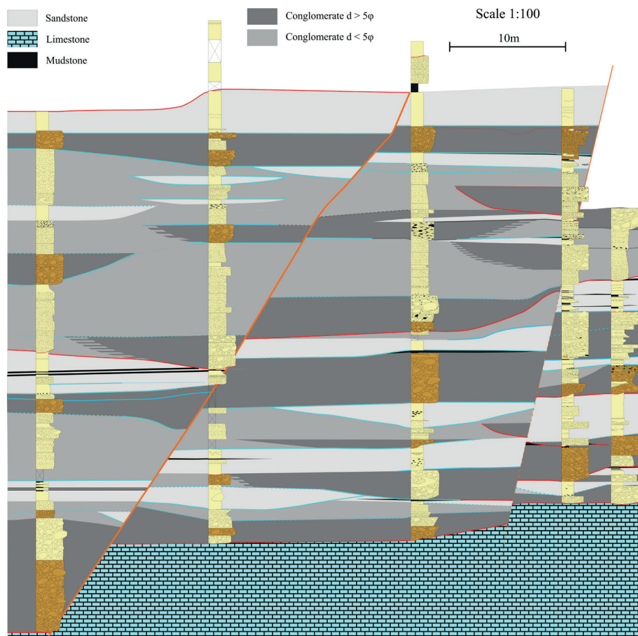
Fig. 22. Correlation of detailed sedimentological logs of Skrzydlina quarry outcrop within five exploitation levels as documented in years 2017–2018. Two main stages of olistostrome deposition are indicated by broad erosional surfaces marked red (modified from Siemińska et al. , 2018, 2020 and interpretation by Wendorff et al. , 2015)
