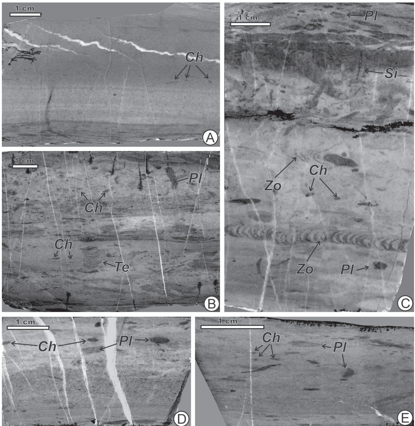
Fig. 39. Trace fossils within Sokolica Radiolarite Fm. in the Flaki Range, Branisko Succession: Ch – Chondrites; Pl – Planolites; Si – Siphonichnus; Te – Teichichnus; Zo – Zoophycos (after Krobicki et al. , 2006)
