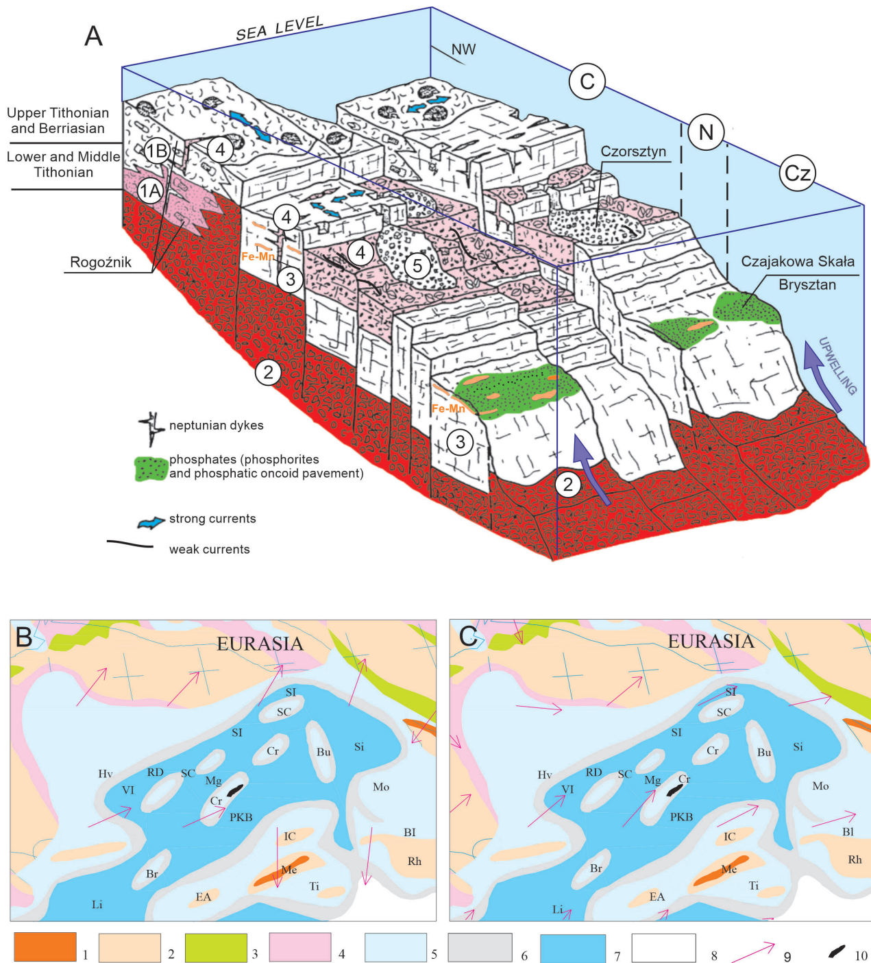
Fig. 31. Model of sedimentation on the intraoceanic Czorsztyn pelagic swell in Berriasian (A) with effects of pronounced Neo-Cimmerian tectonic movements and upwelling currents (after Krobicki, 1996, modified): 1 – Rogożnik Coquina Member (Dursztyn Limestone Formation: A – sparitic coquina, B – micritic coquina); 2 – Czorsztyn Limestone Formation ( Ammonitico Rosso facies); 3 – Sobótka Limestone Member (Dursztyn Limestone Formation); 4, 5 – Łysa Limestone Formation (4 – Harbatowa Limestone Member, 5 – Walentowa Breccia Member); successions: C – Czorsztyn, Cz – Czertezik, N – Niedzica. Palaeoenvironments, wind direction and upwelling zones of the Carpathian area during Tithonian-Berriasian time (palaeogeography after Golonka et al. , 2000, modified): summer Northern Hemisphere (C), and winter Northern Hemisphere (B): 1 – mountains/highlands (active tectonically), 2 – topographic medium-low (inactive tectonically, non-deposit), 3 – terrestrial undifferentiated, 4 – coastal, transitional, marginal marine, 5 – shallow marine, shelf, 6 – slope, 7 – deep ocean basin with sediments (continental, transitional, or oceanic crust), 8 – deep ocean basin with little to no sediments (primarily oceanic crust), 9 – wind directions, 10 – upwelling zone; abbreviations of oceans and plates names: BI – Balcans, Br – Briançonnais terrane, Bu – Bucovinian terrane, Cr – Czorsztyn Ridge, EA – Eastern Alps, Hv – Helvetic zone, IC – Inner Carpathians, Li – Ligurian (Piemont) Ocean, Me – Meliata suture, Mg – Magura Basin, Mo – Moesia Plate, PKB – Pieniny Klippen Belt Basin, RD – Rheno-Danubian Basin, Rh – Rhodopes, SC – Silesian Ridge (cordillera), Si – Siret, Sl – Silesian Basin, Ti – Tisa Plate, VI – Valais Trough
