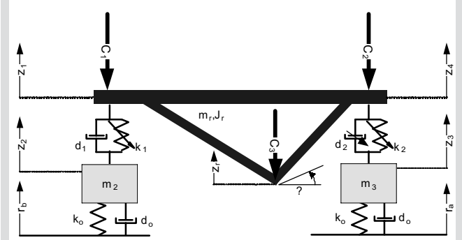
Fig. 2. Bicycle phenomenological model
