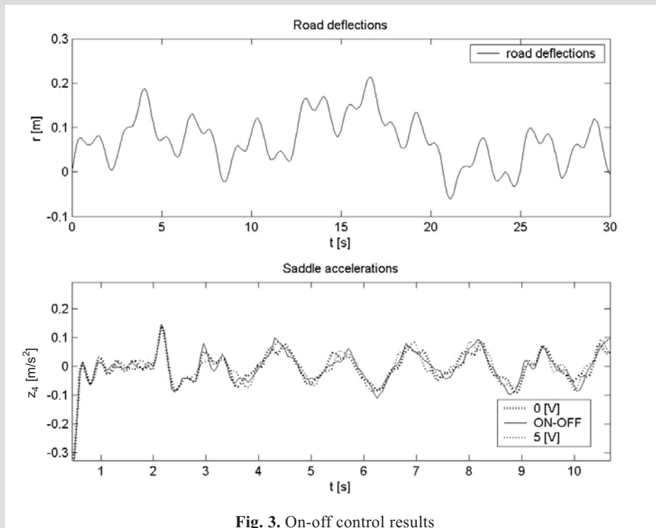
Fig. 3. On-off control results
