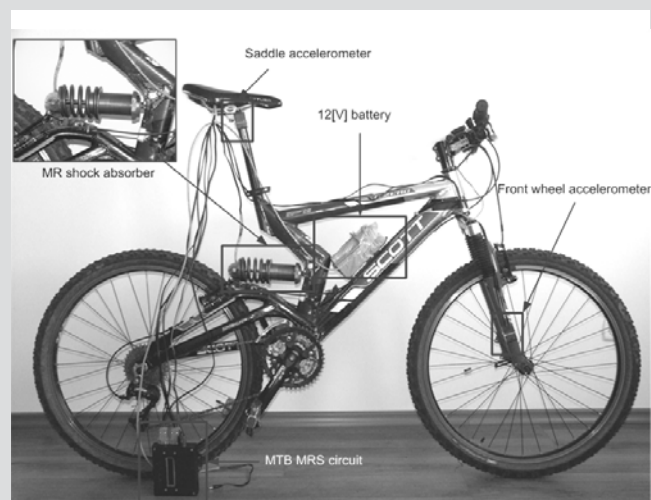
Fig. 1. MR suspension system in a fully suspended bicycle
