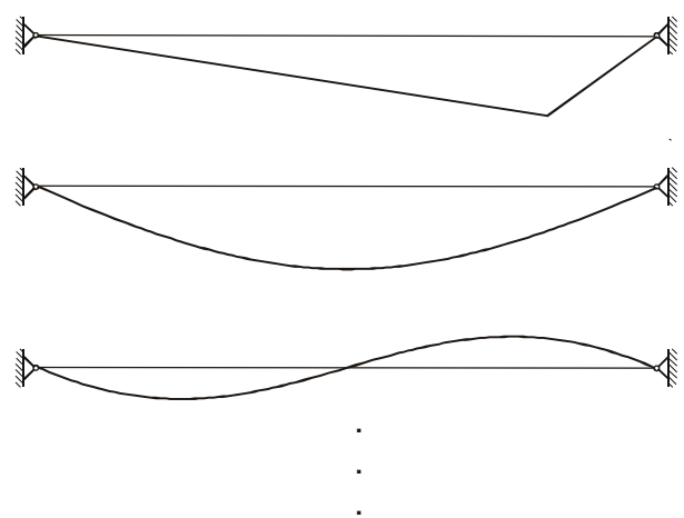
Fig. 7. Selected function used in Ritz-Galerkin method
