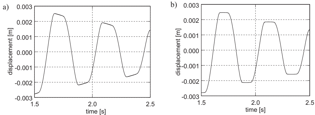
Fig. 13. Displacements of the damper piston: a) hysteresis model; b) Bingham model
