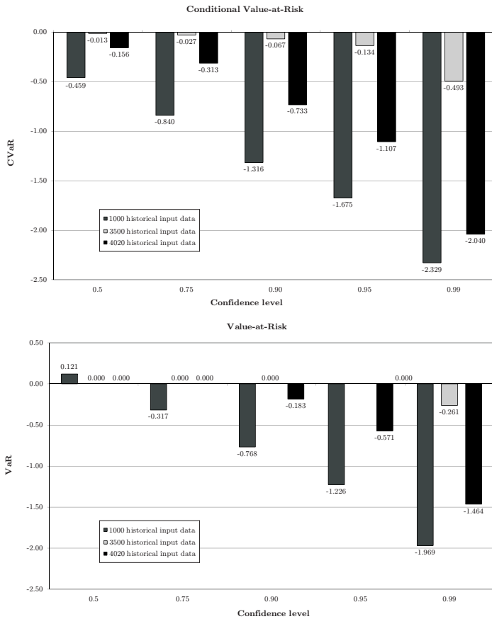
Fig. 2. Comparison of CVaR , VaR and the expected return for CV model with 1000, 3500 and 4020 historical input data
