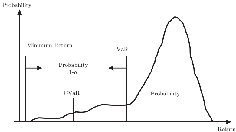
Fig. 1. Value-at-Risk and Conditional Value-at-Risk
