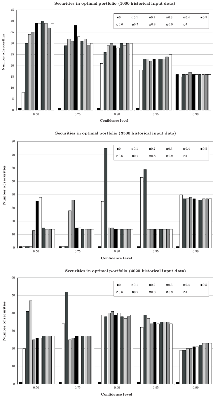
Fig. 7. Number of assets in the optimal portfolio for 1000, 3500, 4020 historical input data – model E_CV
