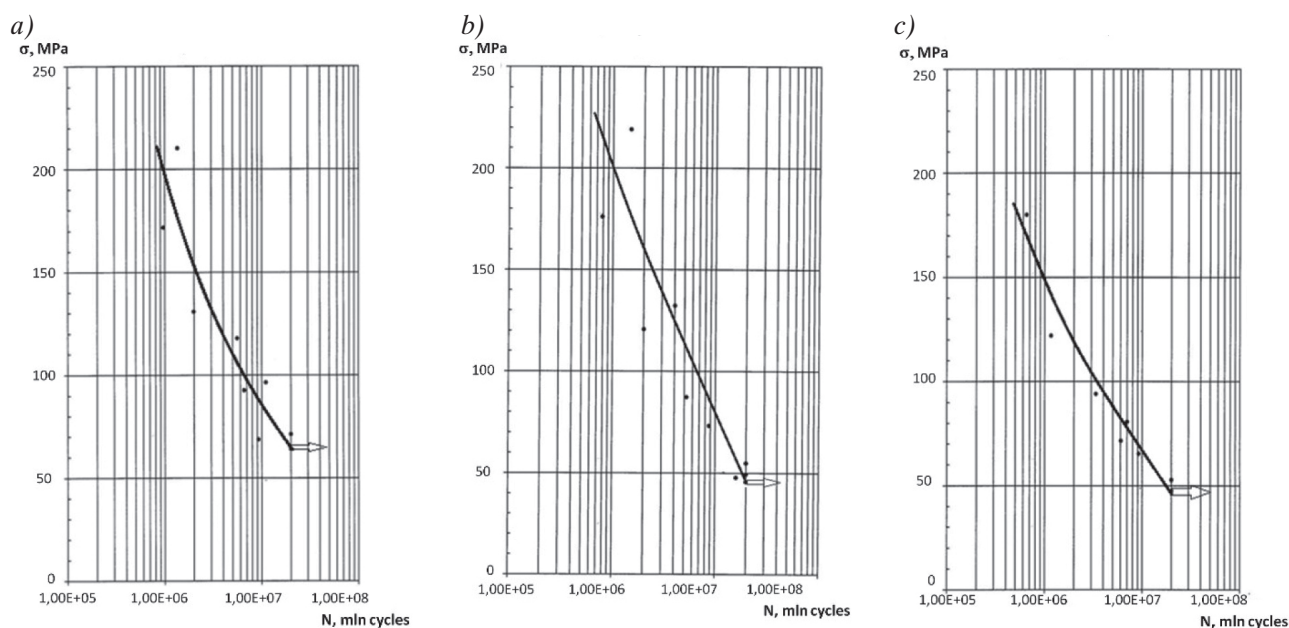
Fig. 2. Corrosion fatigue curve of sucker rod samples with a diameter of 19 mm from steel: a) 15H2GMF when tested in distilled water; b) 15H2GMF when tested in 3% aqueous NaCl solution; c) 15H2GMF when tested in formation water
