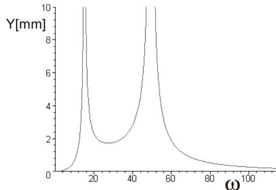
Fig. 13. Amplitude of the frame vibrations of the vibroinsulated vibratory conveyor versus the forced frequency
