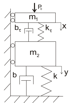
Fig. 3. Simplified scheme of the vibroinsulated conveyor
