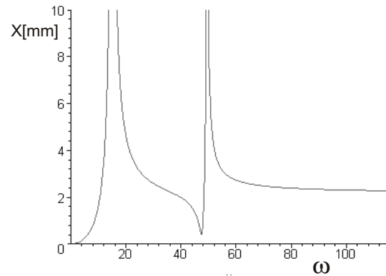
Fig. 12. Amplitude of the trough vibrations of the vibroinsulated vibratory conveyor versus the forced frequency
