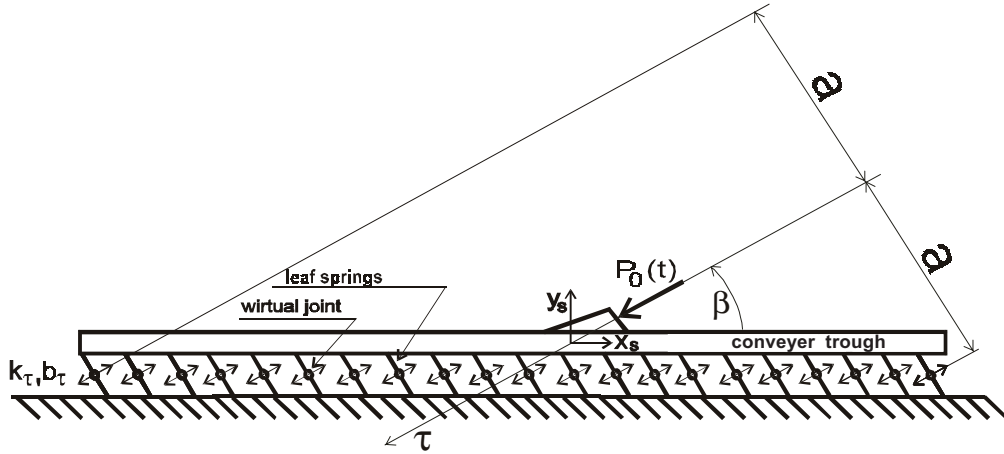
Fig. 1. Model of the vibratory conveyor situated directly on the foundation
