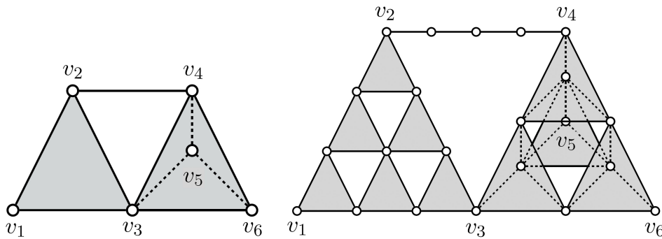
Fig. 2. \mathcal{H} and \mathcal{H}^{\frac{1}{2}}
