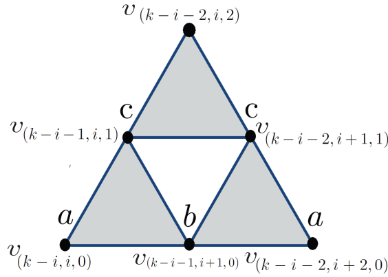
Fig. 3. \mathcal{H} and \mathcal{H}^{\frac{1}{3}}
