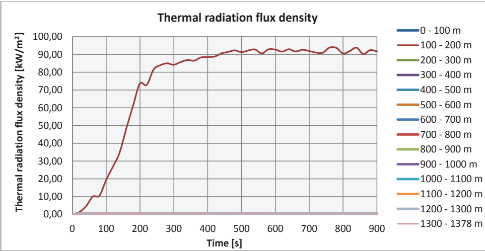
Fig. 9. Thermal radiation flux density
