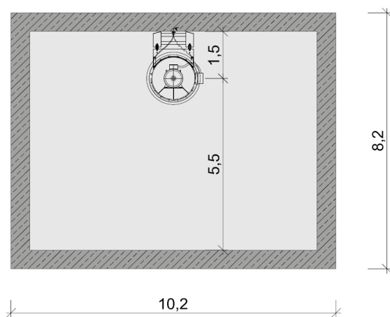
Fig. 3. Tunnel cross-section
