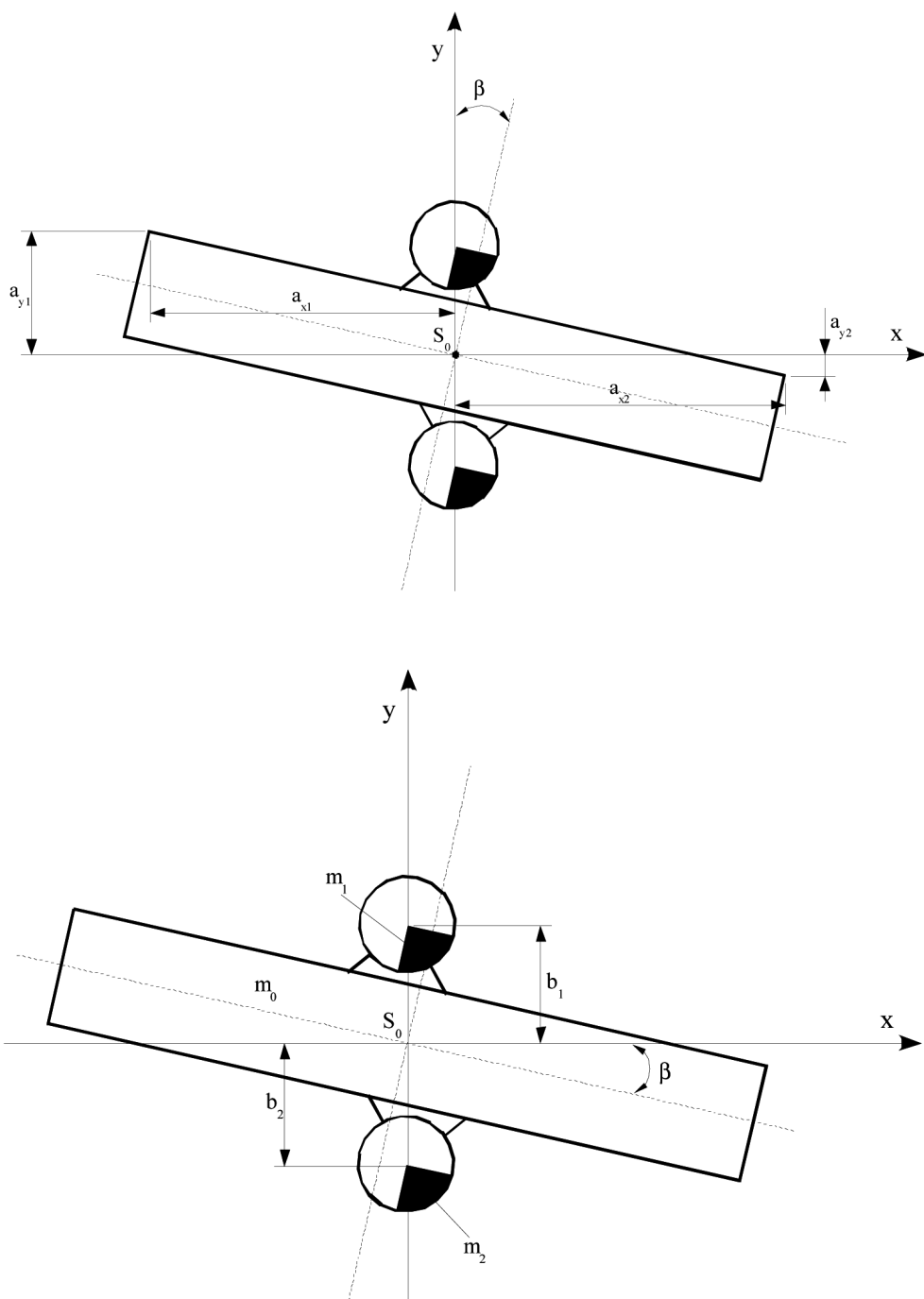
Fig. 2. Markings used for determining sieve motion equations
