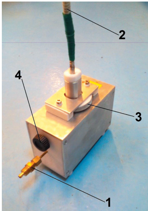
Fig. 5. Measuring chamber: 1 – inlet of measured gas; 2 – fiber-optic armature; 3 and 4 – calibration screws. External dimensions of rectangular part of chamber: 170\text{ mm} \times 100\text{ mm} \times 70\text{ mm}
