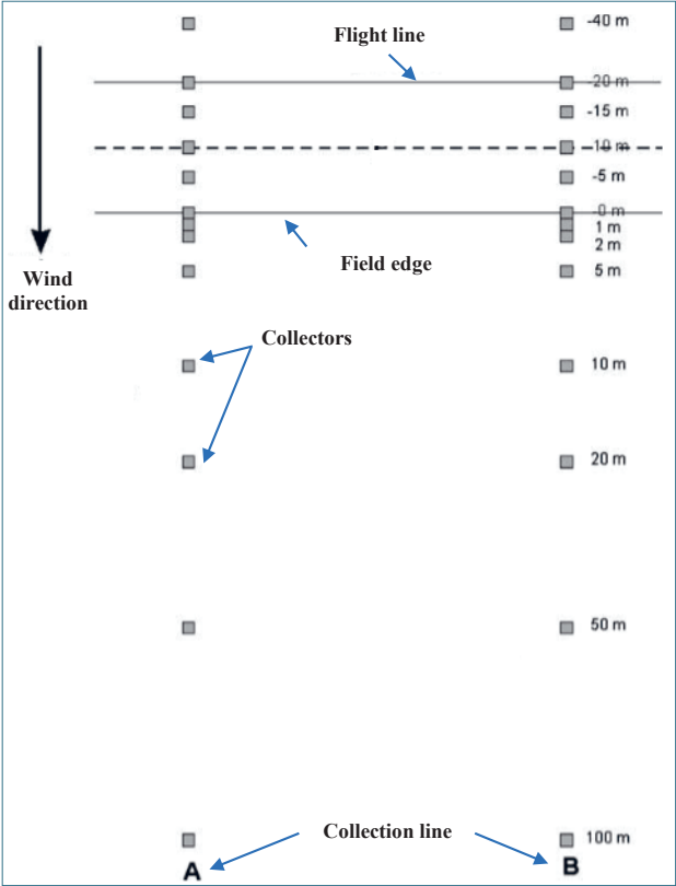
Fig. 6. Arrangement of collectors along collection lines A and B Source: acc. to [43]
