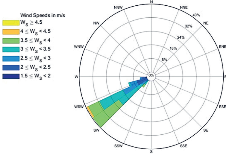
Fig. 4. Wind rose at 10 m in Abidjan, Ivory Coast
