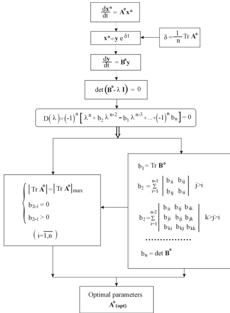
Fig. 4. Algorithm for the optimal selection of control parameters using the Golubencev method
