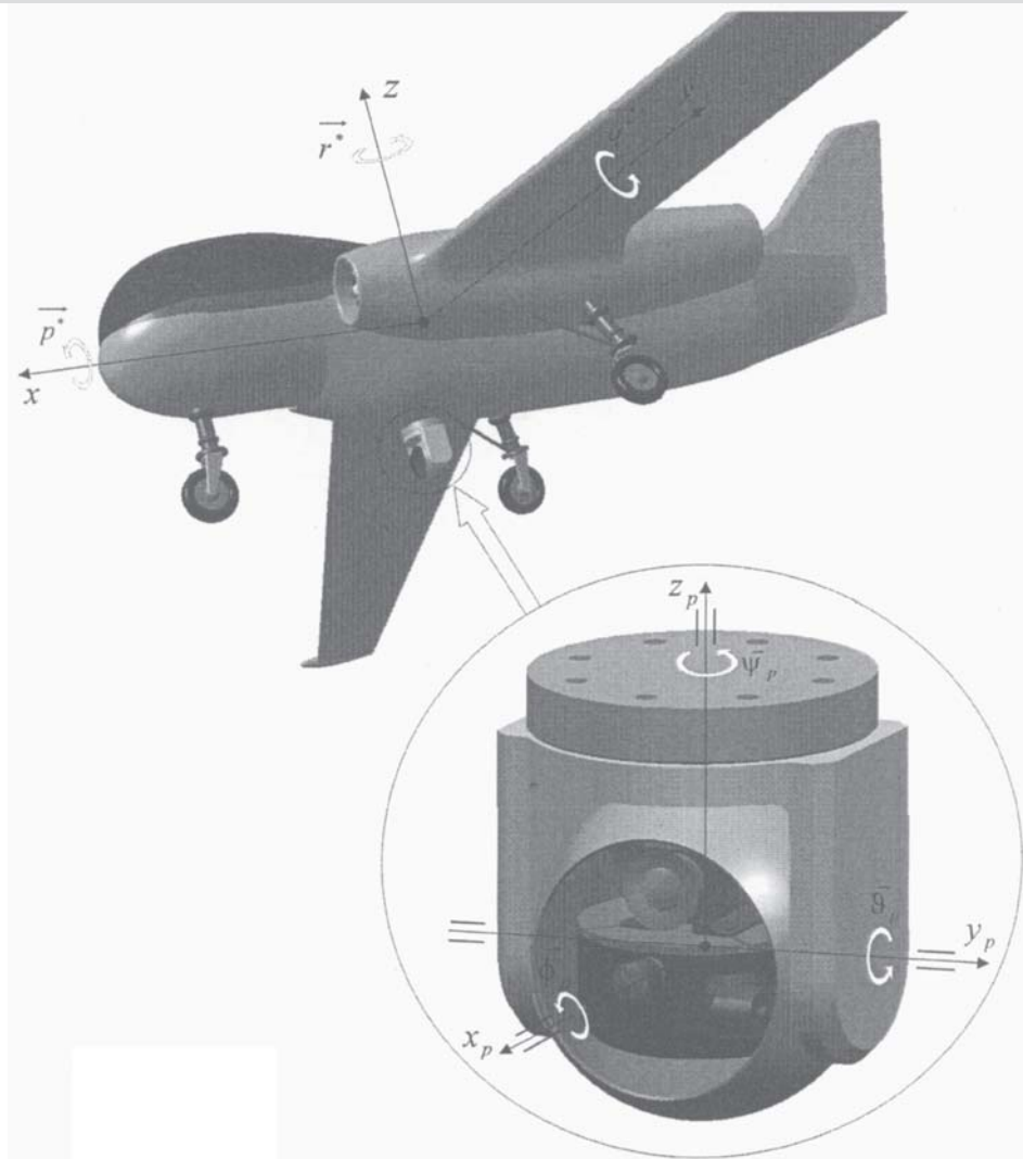
Fig. 1. View of a detecting head stabilised by a gyroscopic platform
